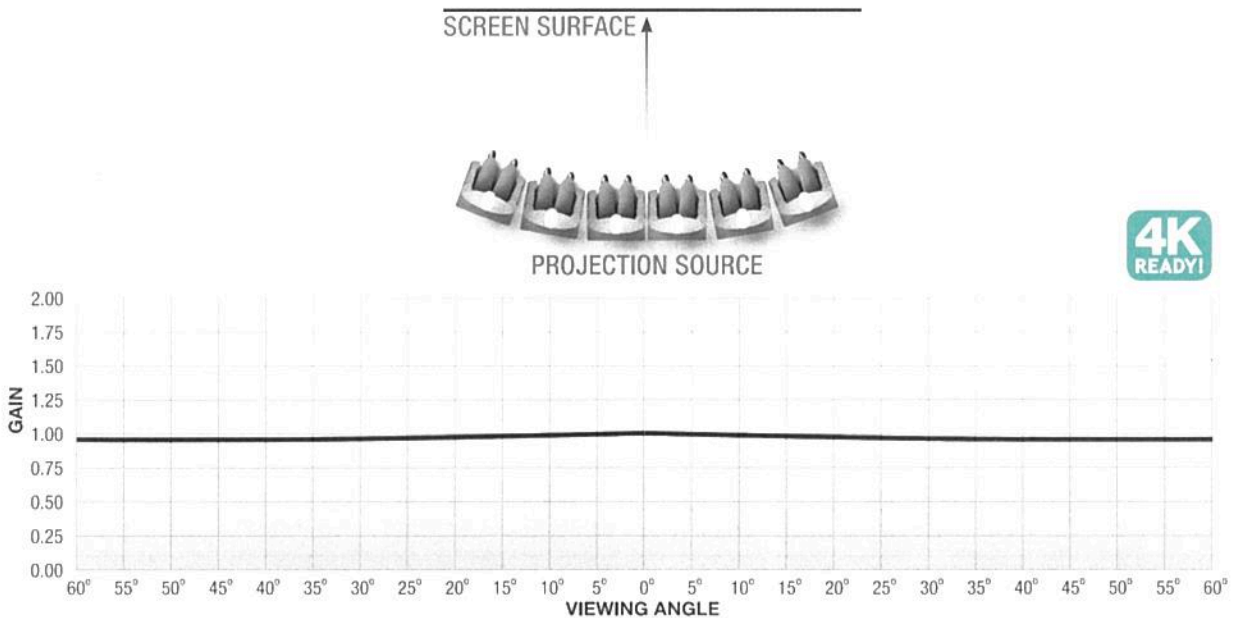
GAIN CHART: 0° GAIN: 1.0, VIEWING CONE: 180° OPTIFLEX MATT WHITE XT1000V
